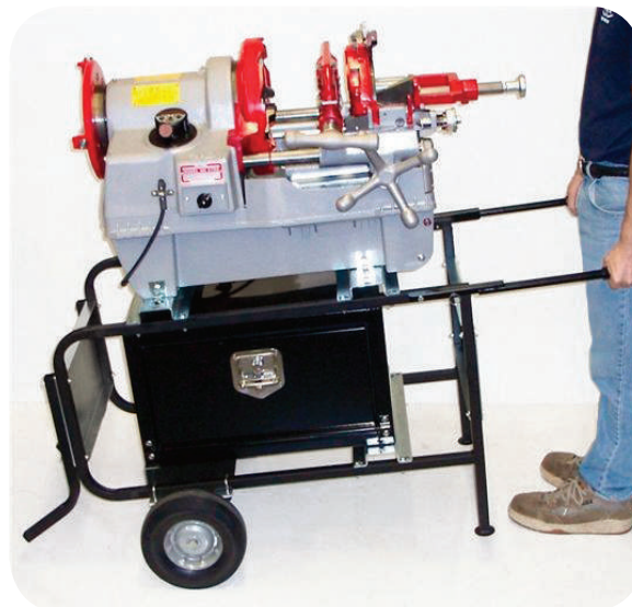
6790 mounted on 60507 cart.
