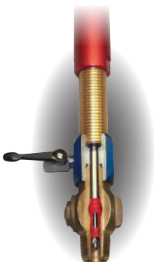
Cutaway View
