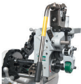
9700 Hydraulic Roll Groover on Threader.
